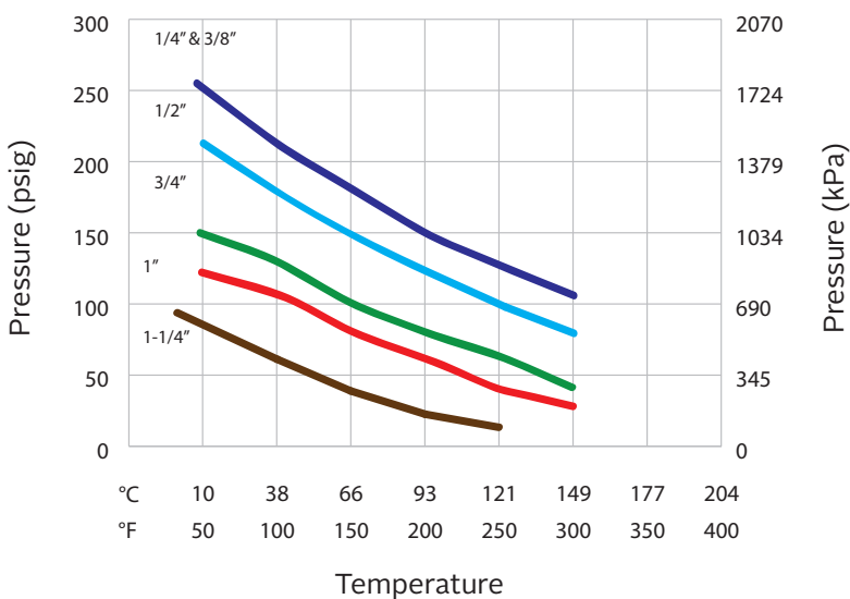
PVDF Fittings Pressure vs. Temperature
